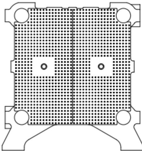
Stationary Platen: Mold Side
