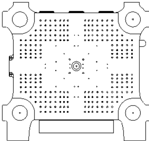
Stationary Platen: Mold Side
