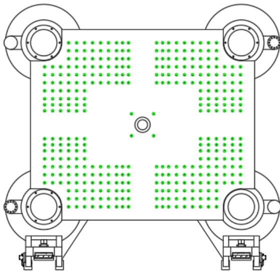
Stationary Platen: Nozzle Side
